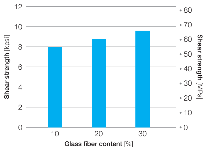
Figure 21: Shear strength of glass-filled Veradel® PESU
