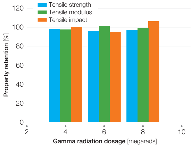
Figure 41: Radiation resistance of Veradel® PESU
