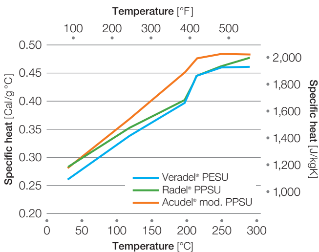
Figure 36: Specific heat
