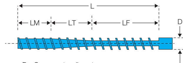
Figure 60: Screw design for injection molding
