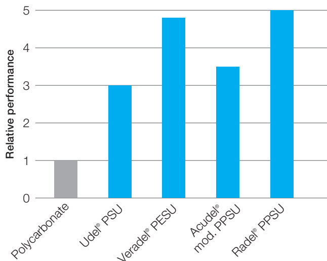
Figure 3: Relative thermal capability of sulfone polymers
