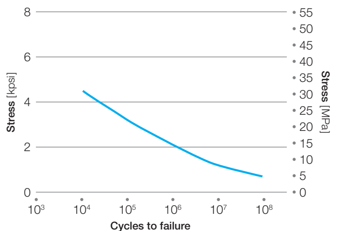
Figure 31: Flexural fatigue endurance of Veradel® A-201 at 30 Hz
