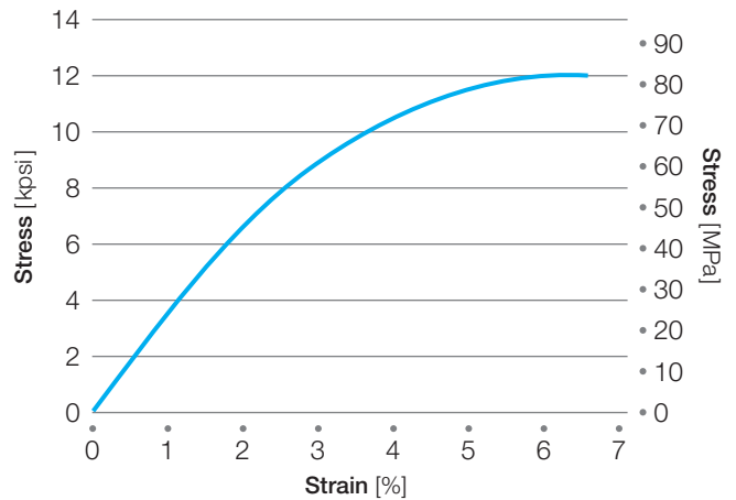
Figure 10: Radel® R-5000 stress-strain curve to yield
