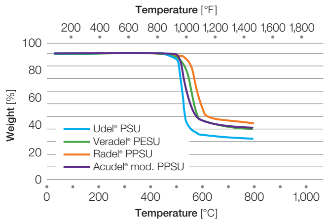
Figure 38: Thermogravimetric analysis in air
