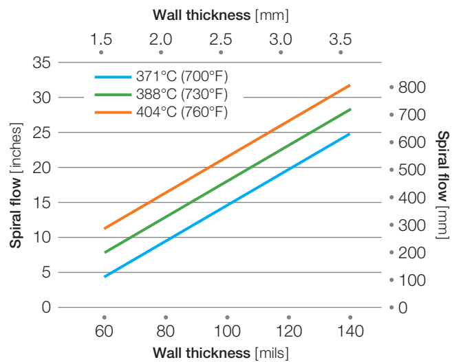
Figure 64: Spiral flow of Radel® R-5800*
