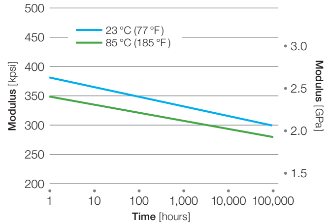
Figure 27: Creep modulus Veradel® A-201 at 20.7 MPa (3,000 psi)
