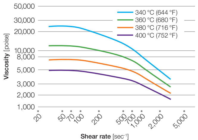
Figure 59: Rheology of Radel® R-5800 resin
