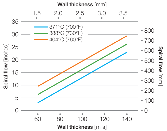
Figure 63: Spiral flow of Radel® R-5000*
