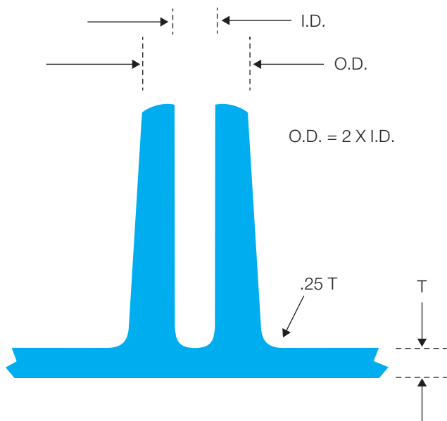
Figure 51: Boss design general guidelines
