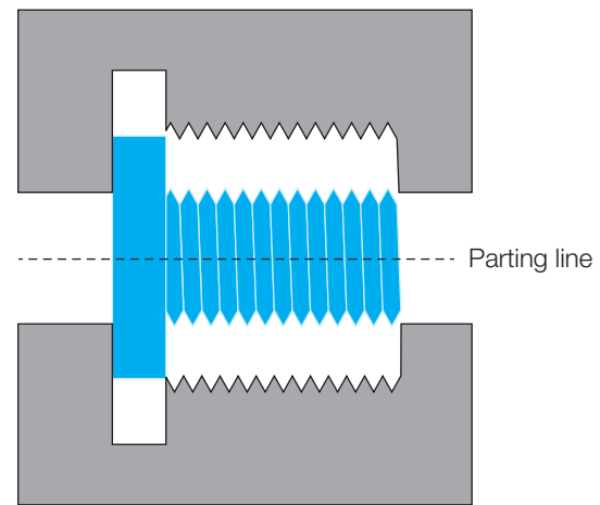
Figure 69: External threads
