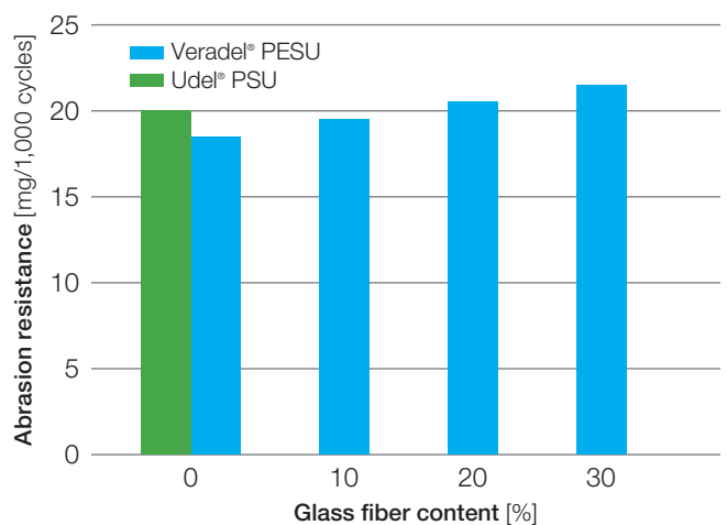
Figure 26: Abrasion resistance
