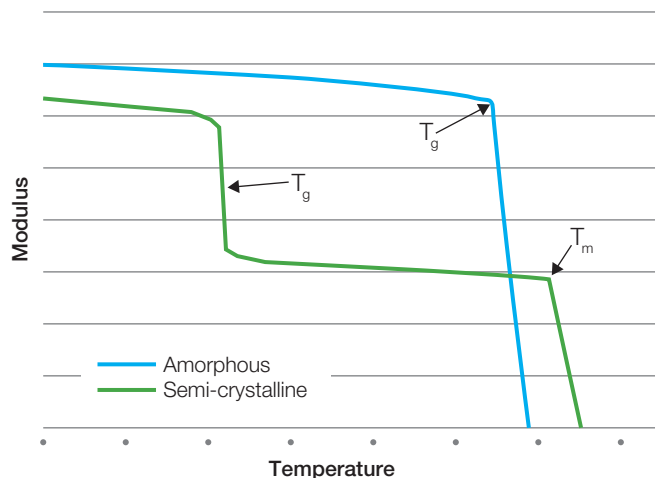
Figure 32: Typical change in modulus with temperature
