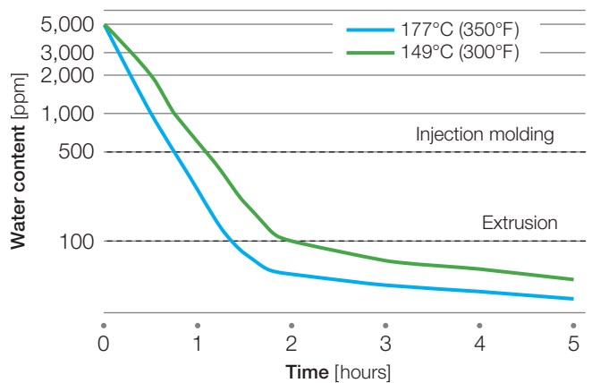
Figure 54: Drying of Acudel® mod. PPSU resin in a circulating air oven
