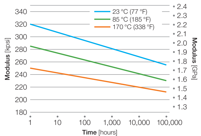
Figure 28: Creep modulus Radel® R-5000 at 20.7 MPa (3,000 psi)
