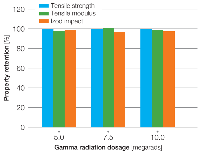
Figure 42: Radiation resistance of Radel® PPSU
