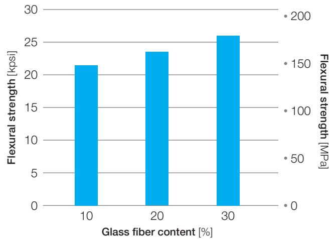
Figure 17: Flexural strength of glass-filled Veradel® PESU
