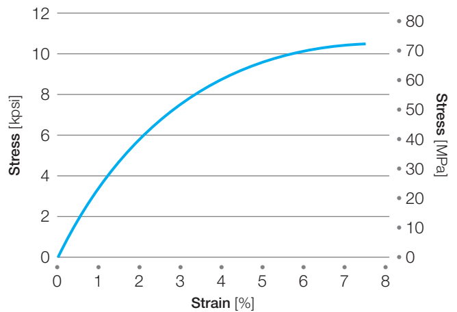
Figure 11: Acudel® 22000 stress-strain curve to yield
