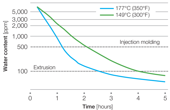
Figure 53: Drying of Radel® PPSU resin in a circulating air oven
