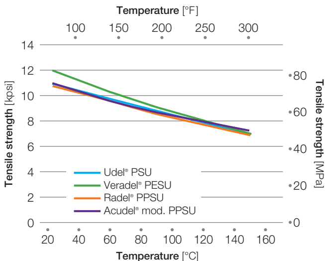
Figure 34: Tensile strength vs. temperature of neat resins
