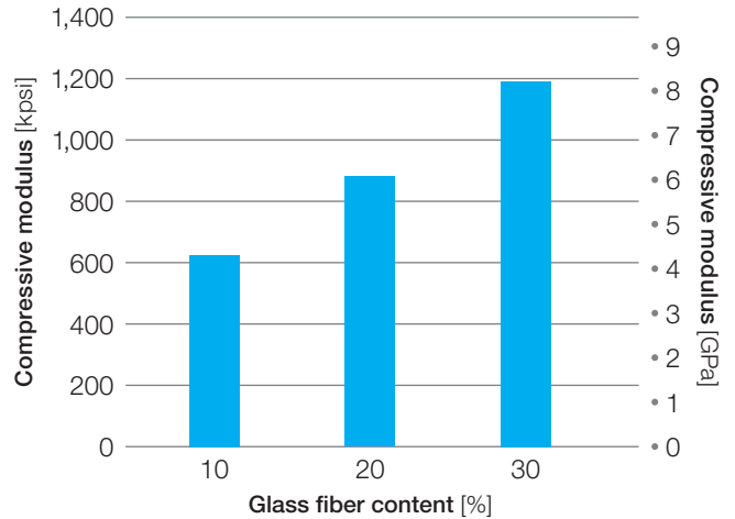
Figure 20: Compressive modulus of glass-filled Veradel® PESU
