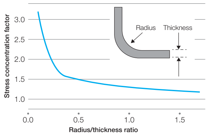
Figure 47: Stress concentration factor at inside corners
