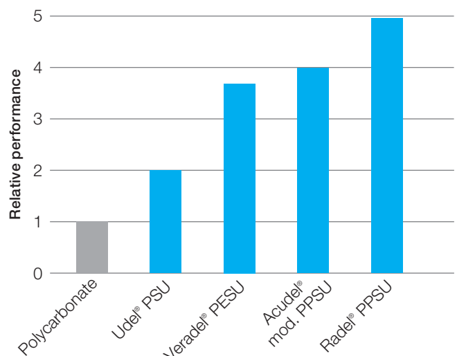
Figure 5: Chemical resistance of sulfone polymers
