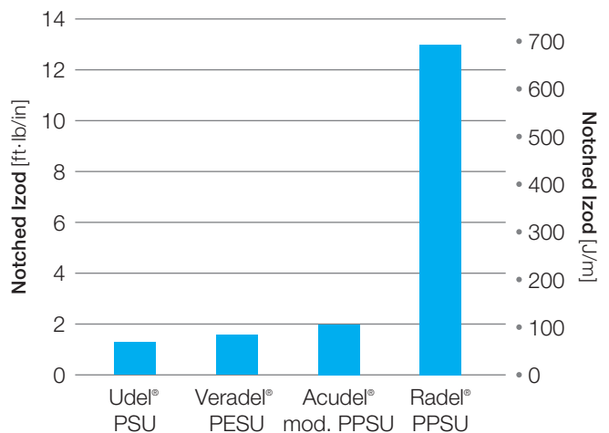
Figure 23: Notched Izod of neat resins
