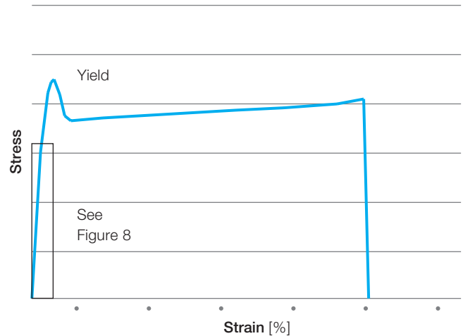
Figure 7: Typical stress-strain curve
