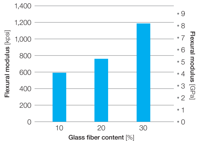
Figure 18: Flexural modulus of glass-filled Veradel® PESU
